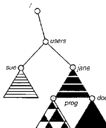
Figure 10.13 Mount point.
