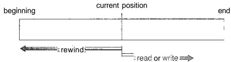
Figure 10.3 Sequential-access file.
