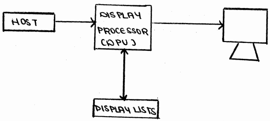
Display-processor architecture
